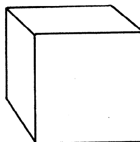
cub
